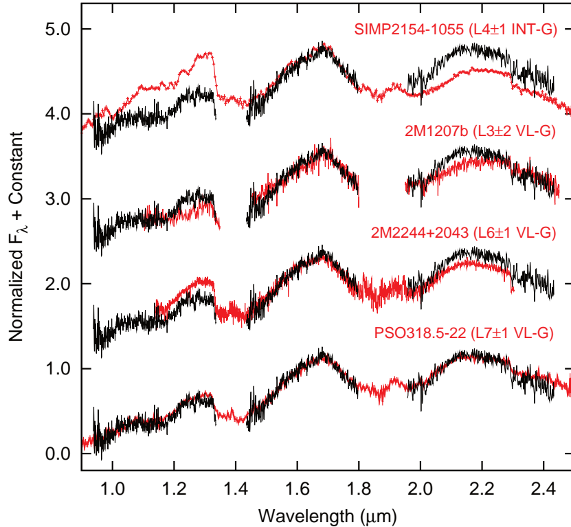
FIG. 7.— SofI/NTT low-resolution near-infrared spectra ( 0.9\text{--}2.4 \mu\text{m} , R \sim 600 ) of the companion VHS 1256-1257 b (plotted in black) compared with an L4 \pm 1 type dwarf SIMP2154-1055 classified as intermediate surface gravity object (INT-G) and with a set of young, very low-gravity (VL-G) L dwarfs (red lines). Spectra were normalized at 1.6 \mu\text{m} and shifted by a constant for display. The spectrum of VHS 1256-1257 b is best matched with spectrum of the free-floating planet PSO J318.5-22 classified as L7 \pm 1 type.
