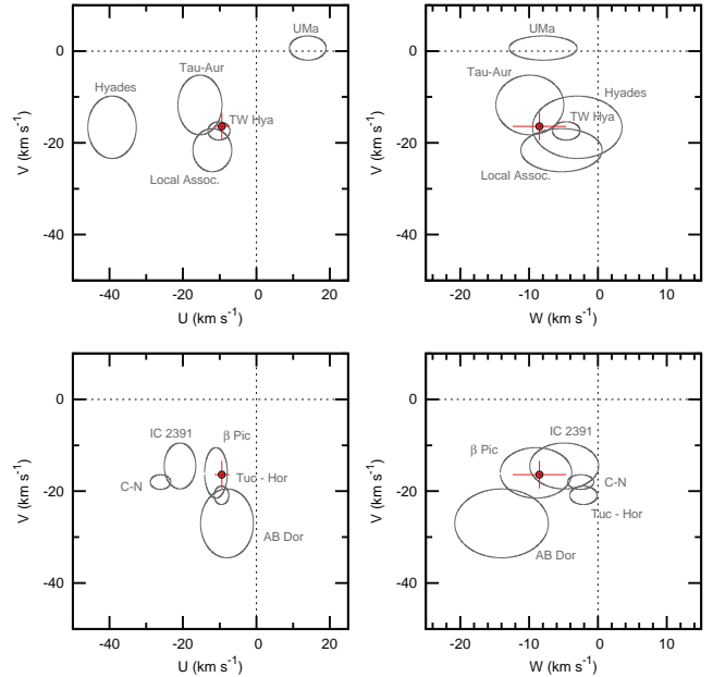
FIG. 9.— Galactic space velocities of VHS 1256-1257 (red dots) with overplotted ellipsoids of known young star associations and moving groups. Errors incorporate uncertainties in the proper motion, parallaxic distance, and radial velocity. Galactocentric U velocity is positive toward the Galactic center.
