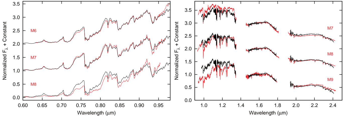
FIG. 4.— Low-resolution GTC/OSIRIS optical (left) and NTT/SofI near-infrared (right) spectra of the primary VHS 1256-1257 plotted with black line, compared with late-M spectral templates (with labels indicating their type). Comparison spectra were smoothed to match the resolution of our data. The sources and references of used templates are described in Section 4.1.1. Spectra were normalized at 0.9 \mu\text{m} at optical and at 1.6 \mu\text{m} at near-IR and offset by a constant for display.
