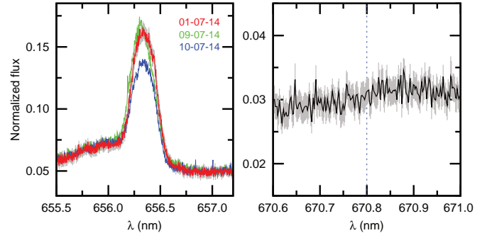
FIG. 11.— Close-up of regions of the VLT/UVES spectrum of the primary VHS 1256-1257, showing, in the left panel the H_\alpha emission line at 656.3 nm and in the right panel the non-detection of lithium absorption at 670.8 nm. Flux uncertainties are plotted in gray.
