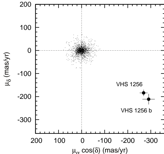
FIG. 2.— Proper motion diagram for the VHS 1256-1257 system. All correlated objects within one degree around the primary with J < 17.5 mag are plotted with black dots. Components of the common proper motion pair are labeled. Error bars correspond to the astrometric RMS of stars near the magnitudes of the components.
