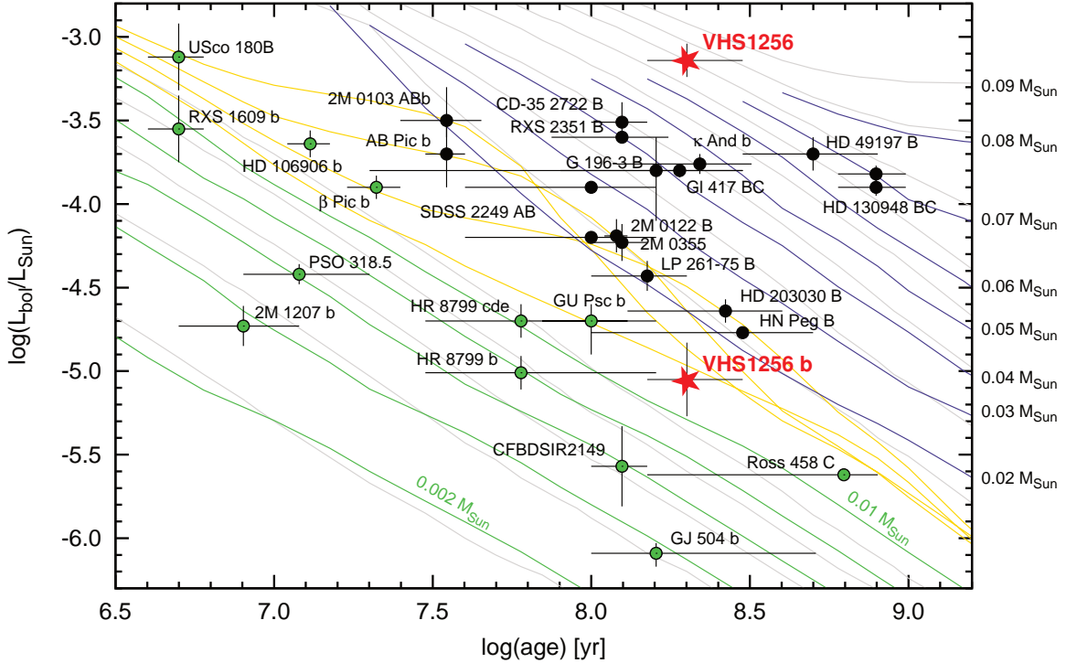
FIG. 13.— Luminosity and age of the two components of VHS 1256-1257 compared with evolutionary tracks from the solar abundance, cloudy atmosphere models of Saumon & Marley (2008) with f_{\text{sed}} = 2 and from the BT-Settl models of the Lyon group (Allard & Barman 2004). The Saumon & Marley (2008) models are plotted in color, with 0.002\text{--}0.010 M_{\odot} tracks in green (spaced by 0.002 M_{\odot} ), 0.011\text{--}0.014 M_{\odot} tracks in yellow with a 0.001 M_{\odot} step, and 0.02\text{--}0.08 M_{\odot} in blue, with 0.01 M_{\odot} increments. The light gray curves correspond to BT-Settl models. For comparison purposes we overplotted the population of known young substellar objects, from the compilations by Bowler et al. (2013), Liu et al. (2013) and updated with recently discovered objects GU Psc b (Naud et al. 2014) and HD 106906 b (Bailey et al. 2014). The BT-Settl isomass lines yield slightly higher luminosities at masses > 0.030 M_{\odot} .
