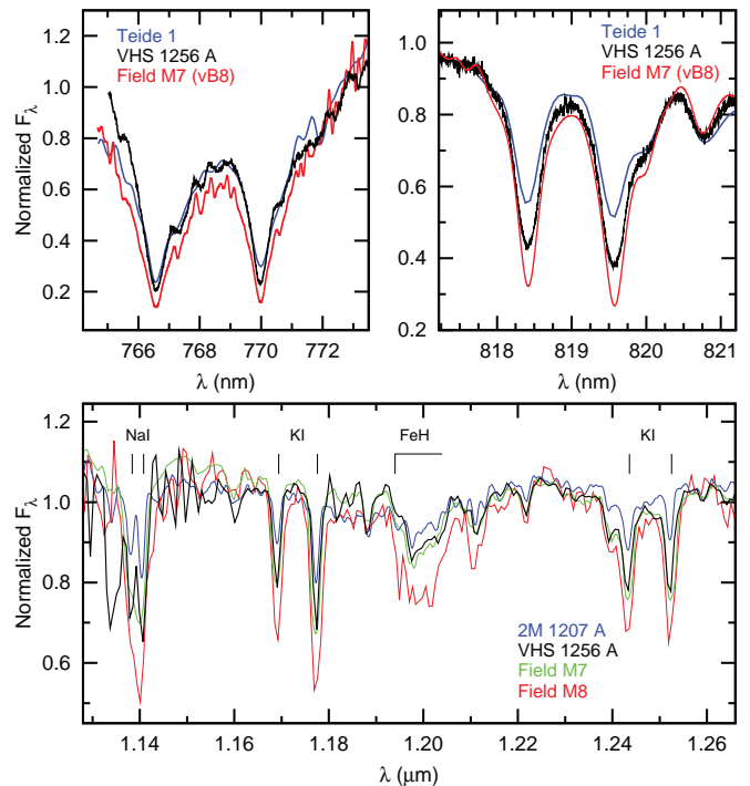
FIG. 5.— Comparison of the Na I and K I lines of the primary VHS 1256-1257 in the optical (top panels) and near-IR (bottom panel) with standard field M7–M8 counterparts and with young low-gravity M8-type dwarfs Teide 1 and 2M 1207 A. All spectra per panel were conveniently normalized at a certain wavelength, and lines were convolved to the same resolution for a proper comparison. These absorption features are slightly less intense than in field objects of similar spectral type.
