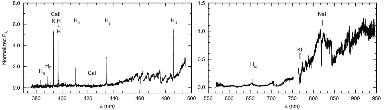
FIG. 10.— VLT/UVES spectra of the primary VHS 1256-1257 covering 373–495 and 565–950 nm wavelength range at a resolution of R \sim 40\,000 ( 25 \text{ m}\text{\AA} \text{ pix}^{-1} ). The blue part of the spectrum (left panel) was smoothed for the display by a factor of 33, degrading the resolution to R \sim 10\,000 . The spectrum has been corrected for telluric absorptions using the ESO Molecfit software. Certain features indicating strong magnetic activity in the chromosphere are visible: the Balmer series emission lines from H_\alpha up to H_\eta , singly ionized calcium H and K lines at 396.85 and 393.37 nm, respectively.
