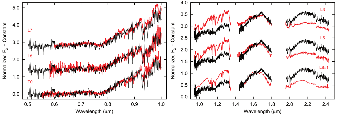
FIG. 6.— Low-resolution GTC/OSIRIS optical (left) and NTT/SofI near-infrared (right) spectra of the companion VHS 1256-1257 b plotted with black line, compared with high-gravity field dwarf templates. The sources and references of used templates are described in Section 4.1.2. Spectra were normalized at 0.9 \mu\text{m} at optical and at 1.6 \mu\text{m} at near-IR and offset by a constant for display.
