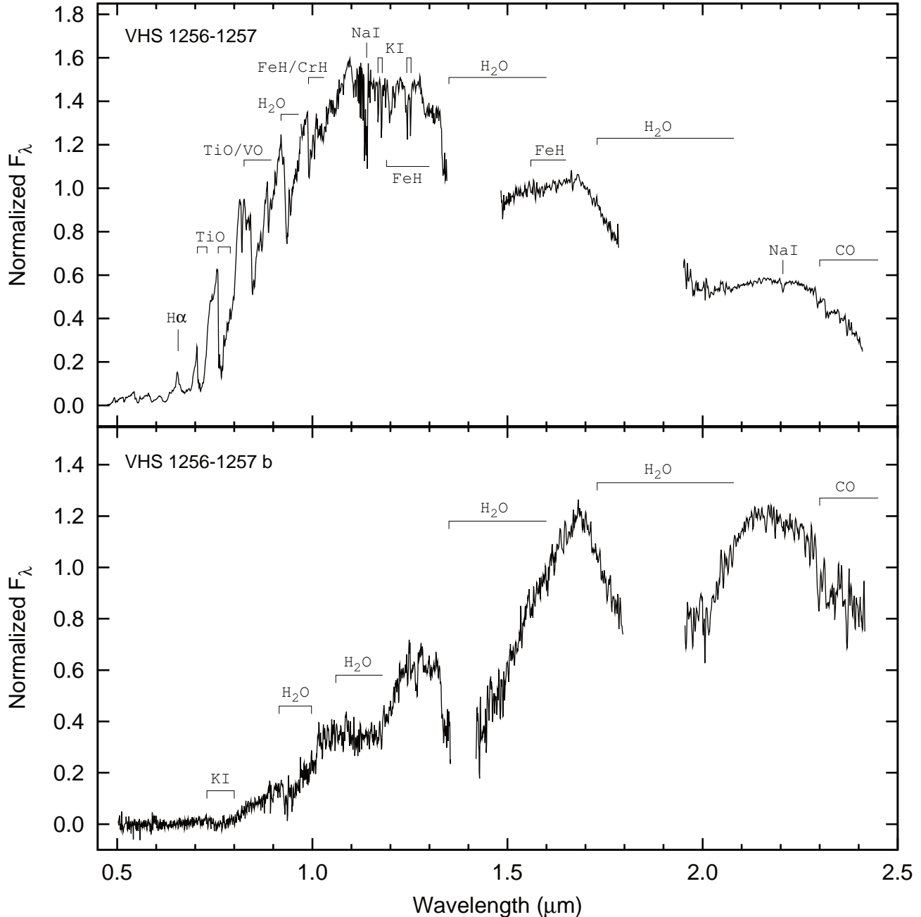
FIG. 3.— Low-resolution optical (0.5–1.0 \mu\text{m} , R \sim 120\text{--}320 ) and near-infrared (1.0–2.4 \mu\text{m} , R \sim 600 ) spectra of the primary (top) and companion (bottom) obtained using GTC/OSIRIS and NTT/SofI. The flux is normalized at 1.6 \mu\text{m} . The most prominent molecular and atomic features are indicated. Unlike most of old population field L dwarfs, the spectrum of VHS 1256-1257 b peaks in the H band, which has a triangle-shaped continuum characteristic for young, dusty L dwarfs.
