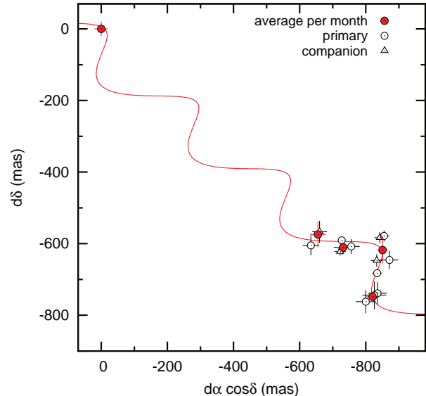
FIG. 8.— Relative apparent trajectory of the components of VHS 1256-1257 in right ascension ( \alpha ) and declination ( \delta ) coordinates for the time interval 2011 July (reference epoch) through 2014 December. Each component is plotted separately as indicated in the figure legend, and the averaged values per observing month are shown with the red solid circles. The solid line indicates the best model fit. North is up and east is to the left.
