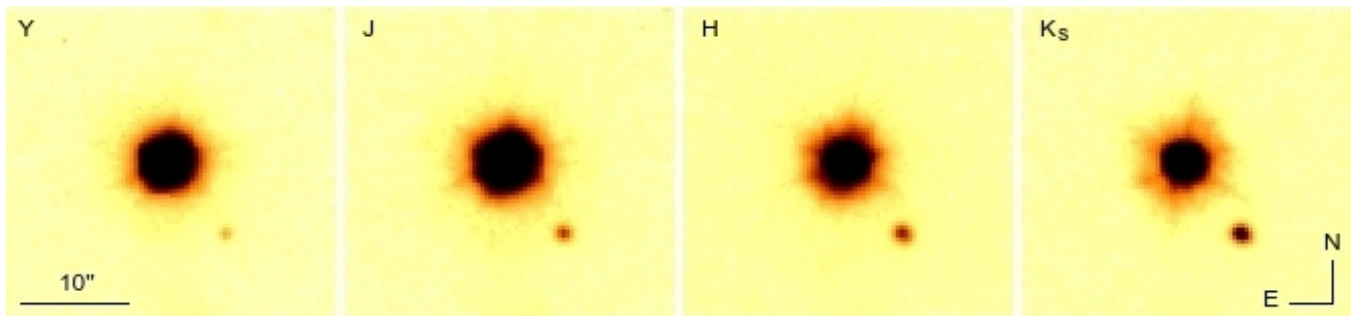
FIG. 1.— VISTA YJHK_s band images of the new common proper motion pair VHS 1256-1257. The identified companion is located at a position angle of 218^\circ.1 \pm 0^\circ.2 , with a projected angular separation of 8''.06 \pm 0''.03 which corresponds to \sim 102 AU at the determined parallactic distance of 12.7 pc. The field of view is 30'' \times 30'' , with north up and east to the left.
